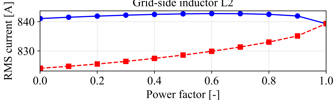
Grid-side inductor L2
